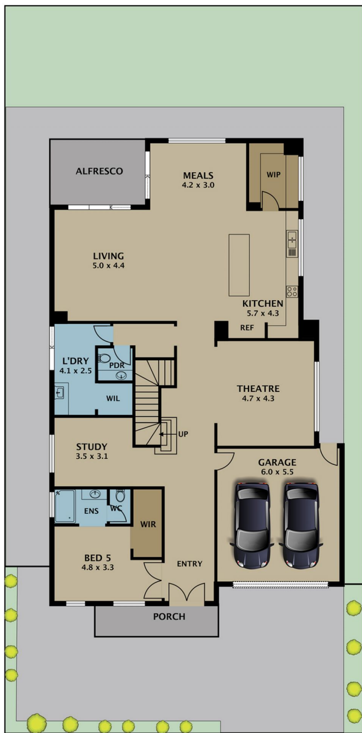
GROUND FLOOR
